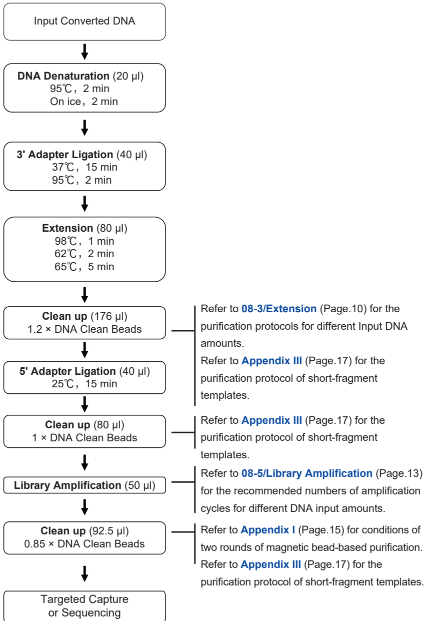
Fig 2. Workflow of EpiArt DNA Methylation Library Kit for Illumina V3
